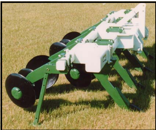
Two Bar Models - Disc gangs bolted to 4" x 4" auxiliary toolbar rigidly clamped to ripper toolbar.
